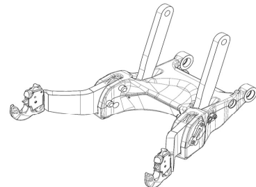
Casting (Part # 72616629)
