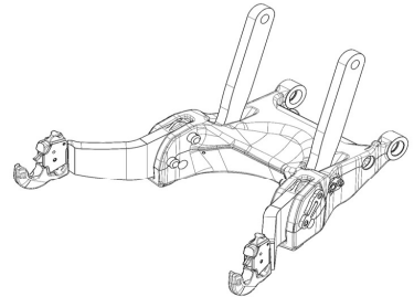
Casting (Part # 72616629)
